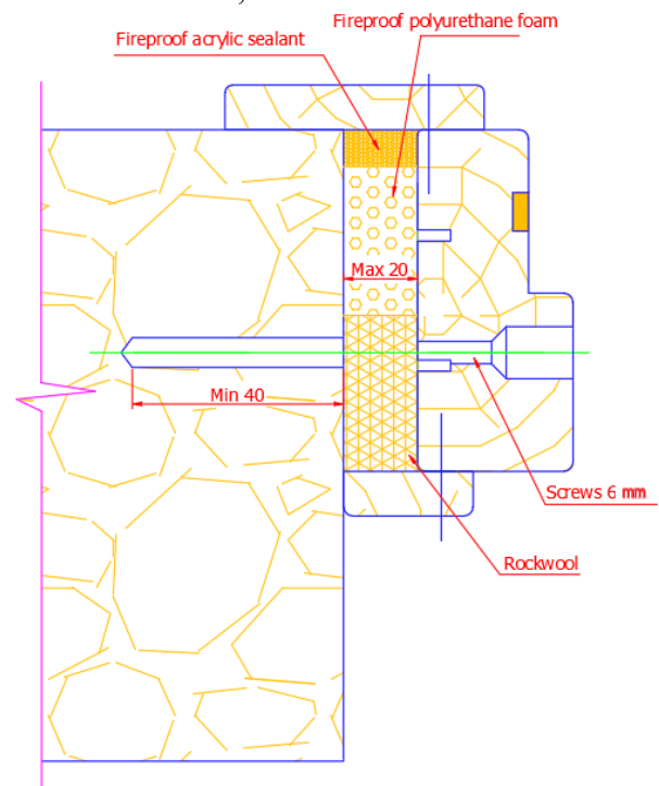
Figure 2. The installation gap between the door frame and the structural opening is filled with mineral wool and fire-resistant urethane foam and sealed on the room side with a fire-resistant sealant
