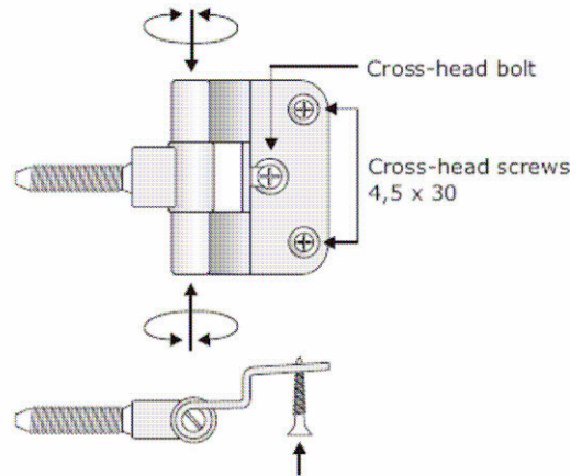
Figure 4. (Adjusting hinges)
